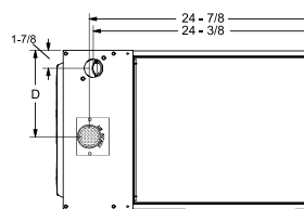
UPFLOW/HORIZONTAL TOP VIEW
